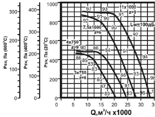
BKPB-9Дy
